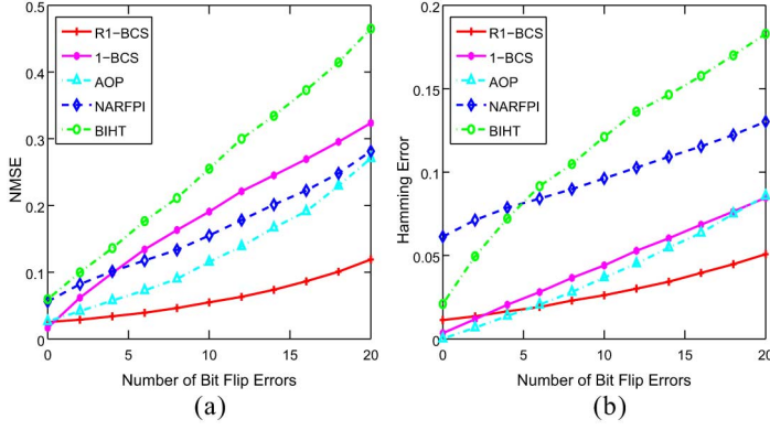
Fig. 2. (a) NMSEs of respective algorithms vs. L ; (b) Hamming errors of respective algorithms vs. L .
