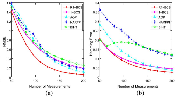
Fig. 3. (a) NMSEs of respective algorithms vs. m ; (b) Hamming errors of respective algorithms vs. m .
