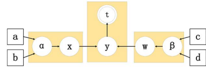
Fig. 1. Hierarchical model for joint sign-flip detection and sparse signal recovery.
